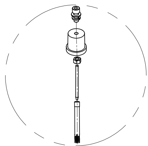
View - A Details Anchor Bolt assembly Enlarged View
